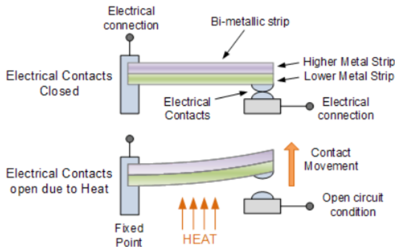
Fig.2.13 Thermal Switch
