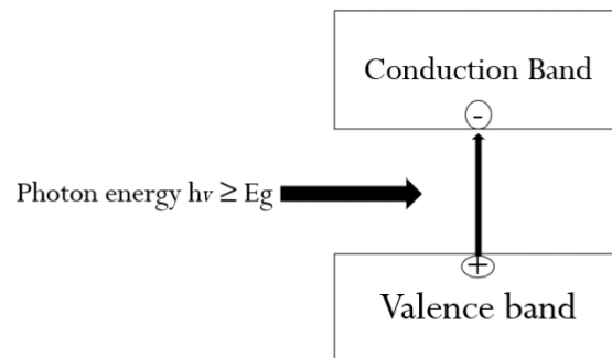
Fig.2.20 Photo conductivity
