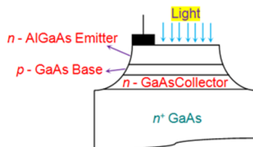
Fig. 2.25 (b) Heterojunction
