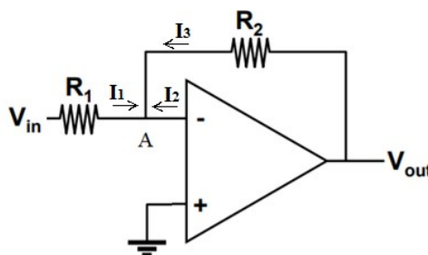
Fig. 4.6 Inverting Amplifier
