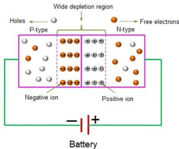
Fig.3.11 Reverse biased PN Junction
