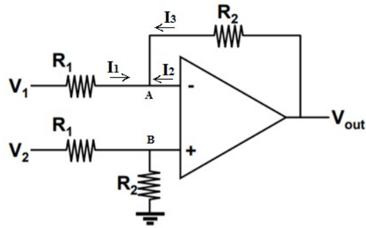
Fig. 4.9. Difference amplifier
